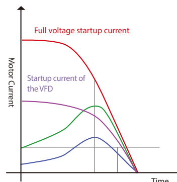
Diagram of changing current from startup to stop
